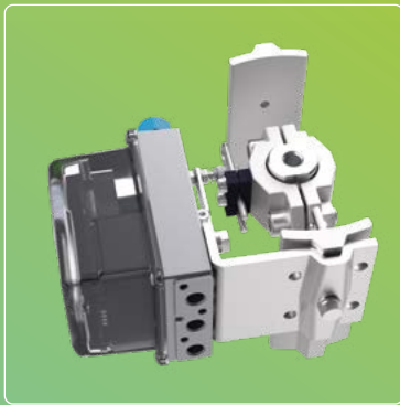
Positioner mounting
